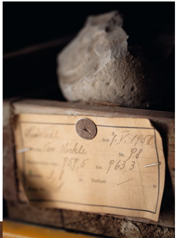
This section of a core from the TECH Center & Lab's archives was drilled in 1958 in Austria. The lab has collected a vast store of cores in its 40 years of existence (top). The holes in this oil-stained cross section of a core originate from previous sample extractions for porosity measurements (left).
